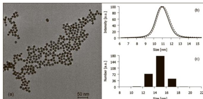
Fig. 1. (a) Low magnification TEM micrograph of Au NPs; (b) particle size distribution in number (–) and volume (–) by differential sedimentation methods, CPS Instruments, Inc. and (c) in number from TEM micrographs.
