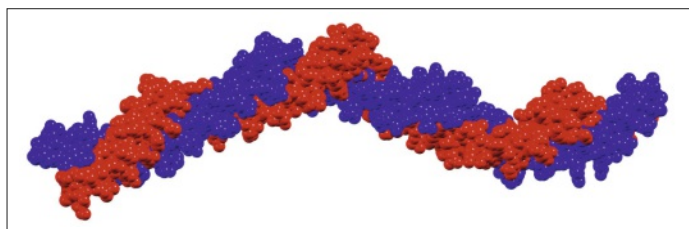
Fig. 3. Representation of a coiled-coil protein containing two strands (PDB code 1C1G [6] ).
