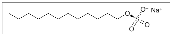
Scheme 4. Structure of sodium dodecyl sulfate.
