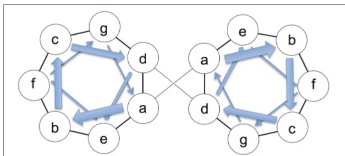
Scheme 2. Heptad wheel representation of a coiled-coil dimer with the helical polypeptide chains in a parallel orientation. The arrows show the direction of the helical twist around each abcdefg -unit which repeats along the chain.
